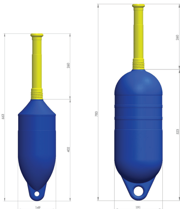
T-5 TRAP BUOY 6 X 11
